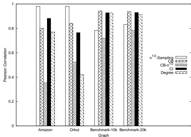
Figure 5: The Pearson correlation of five betweenness approximation algorithms against the actual betweenness on four networks. CB corresponds to our approximation and CB - n^{1/2} corresponds to \sqrt{n} sampling on the Focused Abstract Graph. Results are averaged over 10 realizations.
