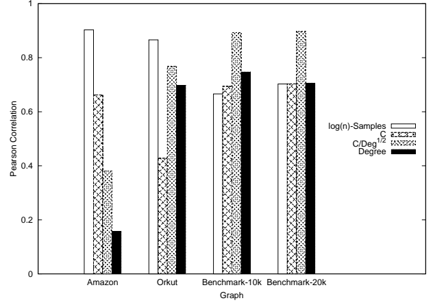
Figure 3: The Pearson correlation of four closeness approximation algorithms against the actual closeness on four networks. \widehat{C}_C is denoted by C and \widetilde{C}_C by C/Deg^{1/2} . Results are averaged over 10 realizations.
