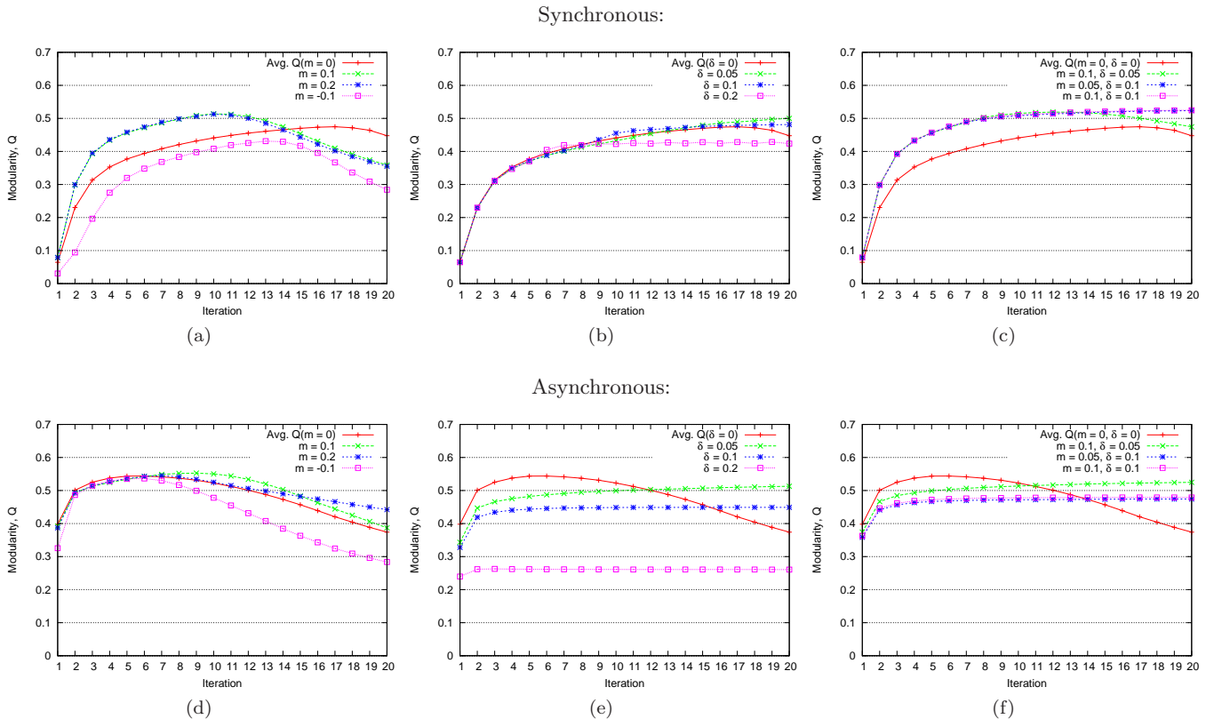
FIG. 8: Average performance comparisons of the synchronous and asynchronous implementations with varying \delta and m over 5 Runs.
